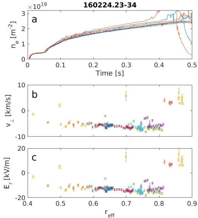
FIG. 5: Line averaged density (a) of a series of discharges. The v_\perp and related E_r as function of r_{\text{eff}} . The different colours indicate the different discharges. Note the change in sign at the plasma edge.
